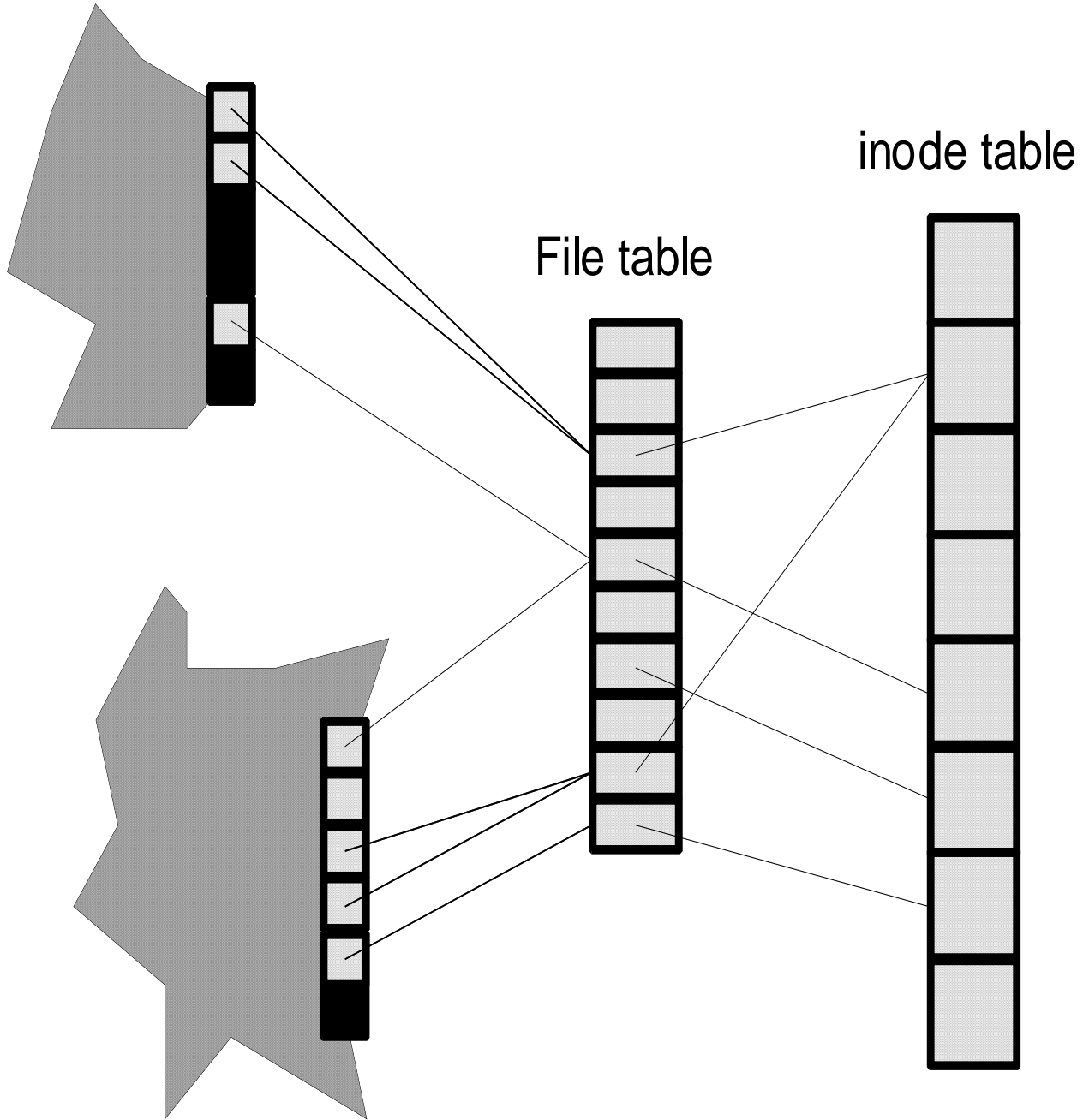
Figure 4. Kernel data structures for open files
